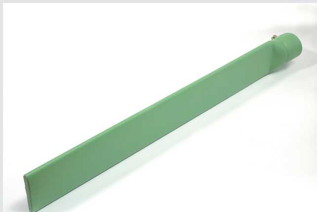
Sword-shaped nozzle (edges rounded) 74 x 12 x 520 mm, PTFE coated Article No: 107.347
