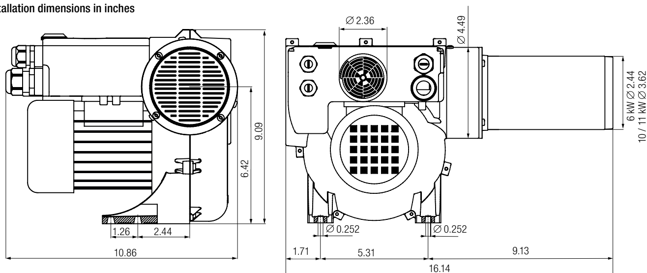
Installation dimensions in inches
