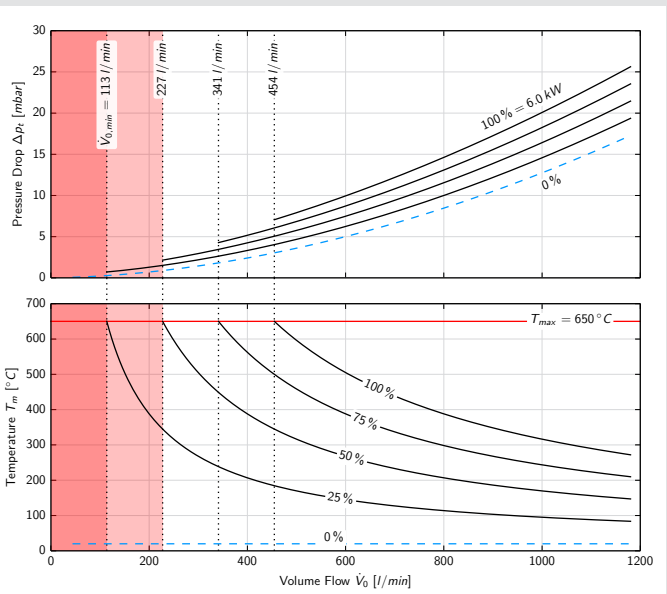
Example of pressure loss and temperature curves for an LHS 61S SYSTEM (3 x 400 V / 6 kW) air heater.
