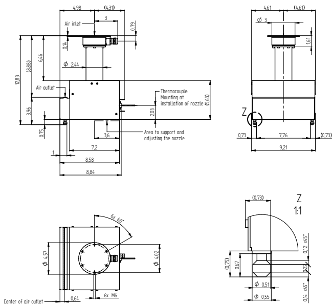
Installation dimensions in inches LE 5000 HT-U
